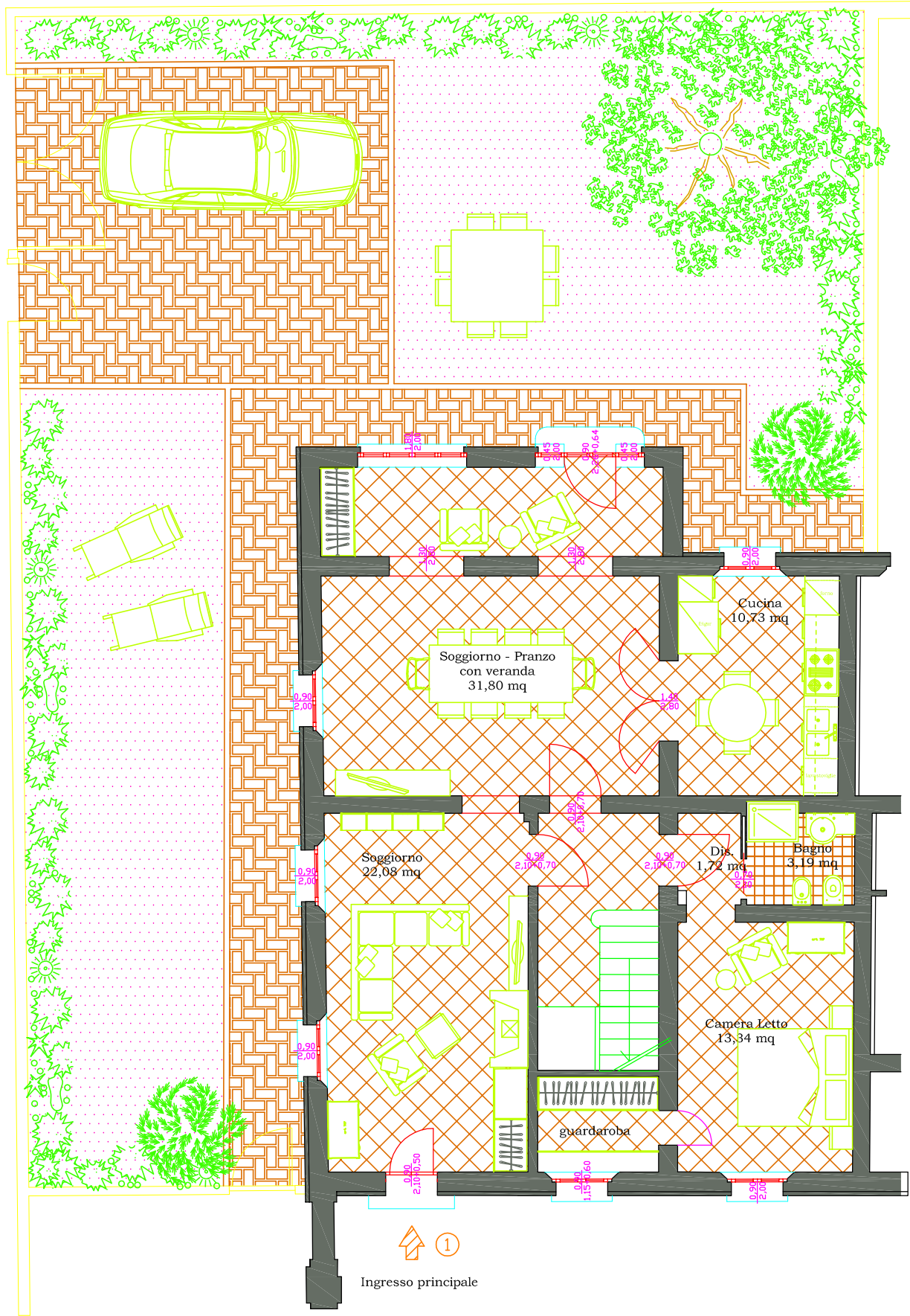
PIANO TERRA
