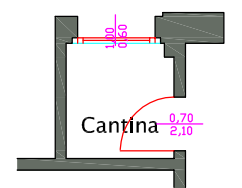
PIANO TERRA
