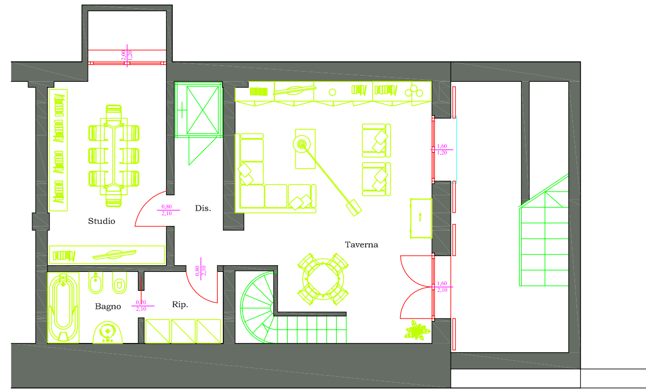
PIANO INTERRATO
