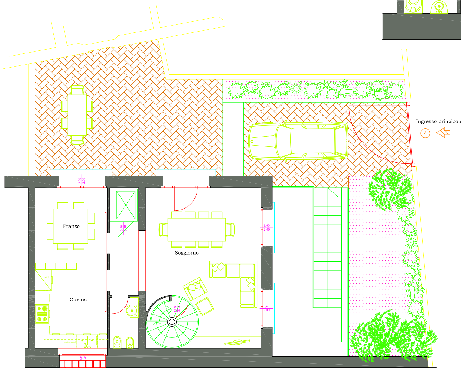
PIANO TERRA
