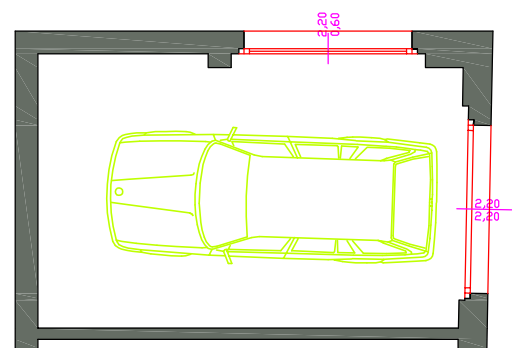
PIANO TERRA
